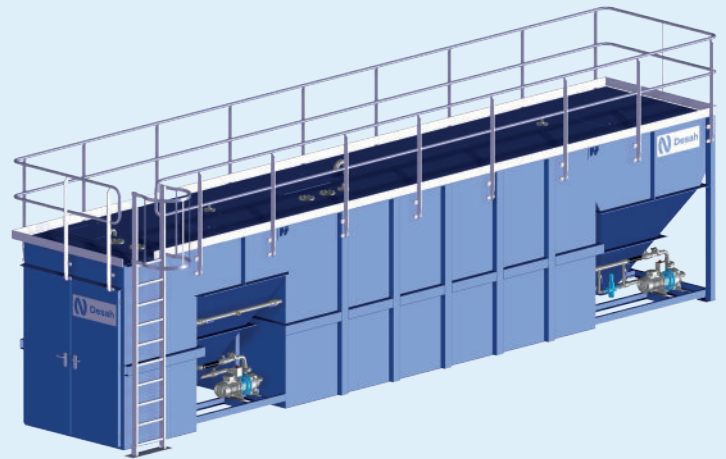
Adsorption/Bio-oxidation system
